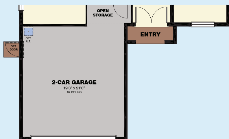
FIRST FLOOR PLAN ELEVATION 'C' VARIATION
