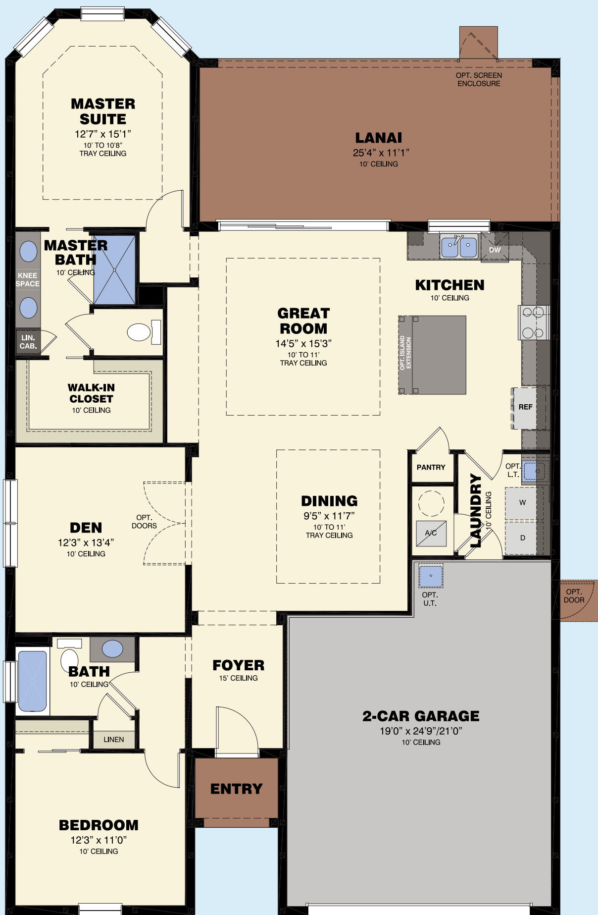
FLOOR PLAN
